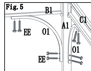
Fig.5:Attach arc support(O1) to post(A1) and across screen(B1, C1), by using bolt(EE).
