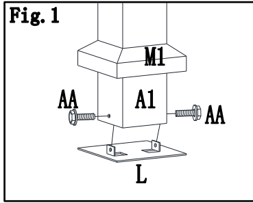
Fig. 1: Put stake cover (M1) through Post(A1) and lift up stake cover, then attach stake slate (L) to bottom of post (A1) by using bolt(AA).
