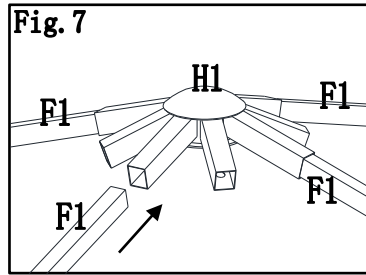
Fig.7 : Insert slanting beam(F1) into big top connector(H1).
