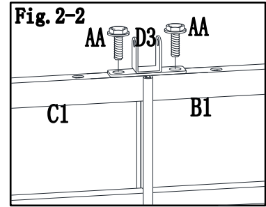
Fig.2-2: Attach middle beam lower connector(D3) to long screen(B1) and short screen(C1), by using bolt(AA).
