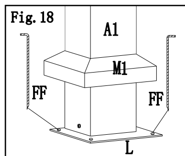
Fig.18 : By using stake(FF) fix assembled gazebo on ground.
