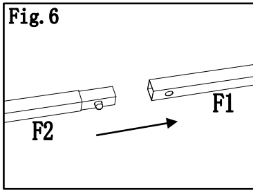
Fig. 6 : Insert the inclined beam down tube (F2) into the inclined beam (F1) and snap the spring buckle on the inclined beam down tube (F2) to the inclined beam (F1) Fixed in the hole position.
