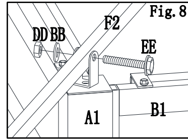
Fig.8: By using bolt(EE),washer (BB),nut(DD), attach slanting beam lower bar(F2) to post (A1).
