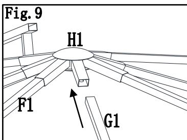
Fig.9: Insert middle beam(G1) to big top connector(H1). Then screw the hook(E1) to big top connector(H1).
