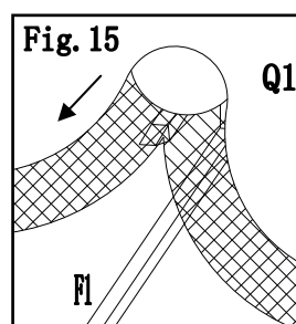
Fig.15: Fix middle canopy four corner (Q1) to big top slanting beam upper bar ( F1 ),then adjust middle top end tube till middle canopy tight.
