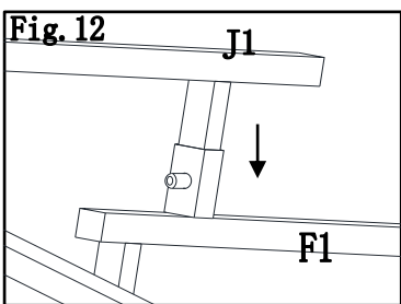
Fig.12: Put large canopy(R1), middle canopy(Q1) on top. Then insert assembled small top slanting bar(J1) into big top slanting upper bar(F1).
