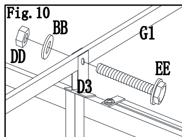
Fig.10: By using bolt(EE), washer(BB),nut(DD),attach middle beam(G1) to middle beam connector(D3).
