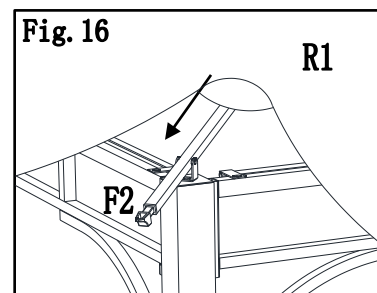
Fig.16 : Fix big canopy four corner(R1) to big top slanting lower bar (F2), then adjust big top end tube till canopy tight.
