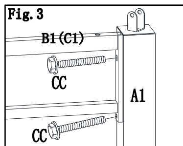
Fig.3: Then fix assemble screen(B1,C1) to post(A1) by using bolt(CC).
