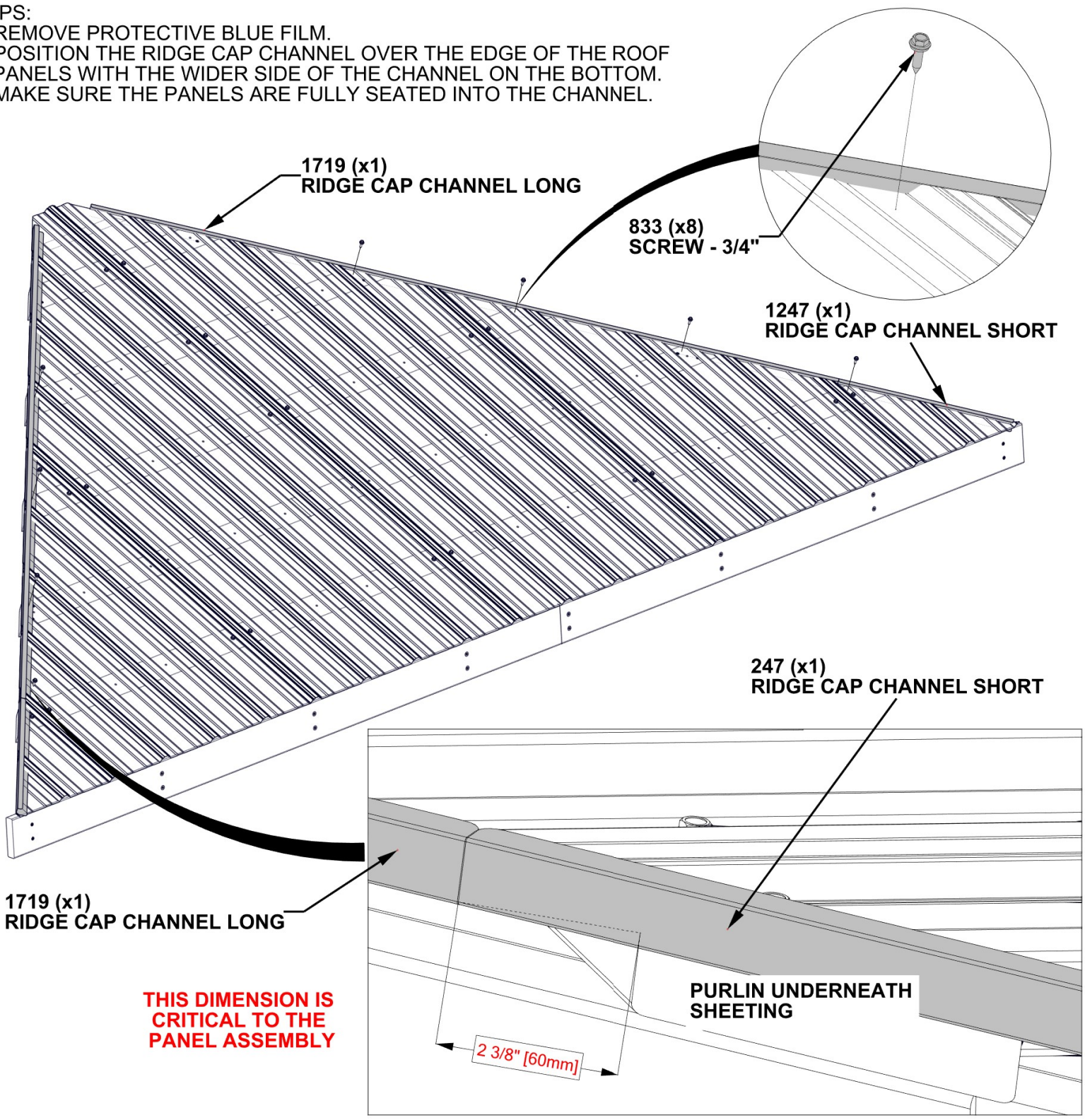
A4M01719 RIDGE CAP CHANNEL LONG (x2)
