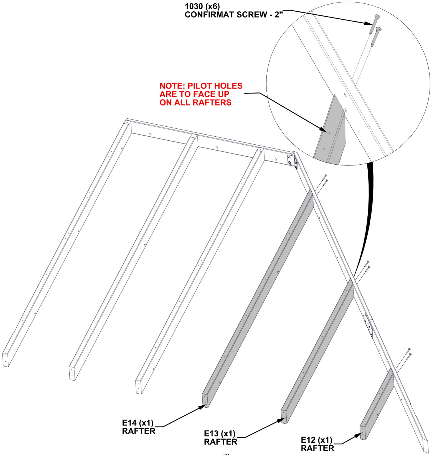
E14 RAFTER - W4L17567 (x1) 1 7/16"x3 3/8"x67 1/8" (36x86x1705)
