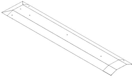
A4M01900 RIDGE PEAK CAP (x1)
